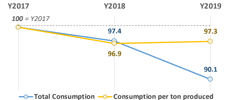
<Chart 1 - Energy Consumption>
